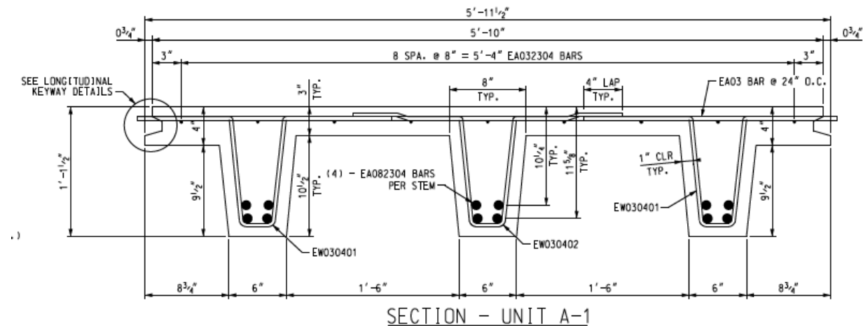
Figure 5: Individual panel cross-section
