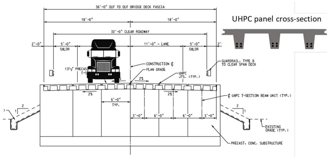
Figure 4: Cross-section of novel UHPC deck bridge
