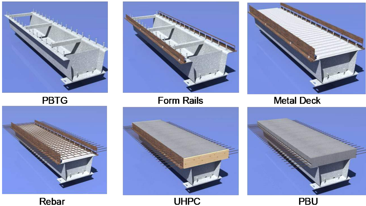
Figure 1: Construction of composite UHPC/ PBTG prefabricated bridge unit
